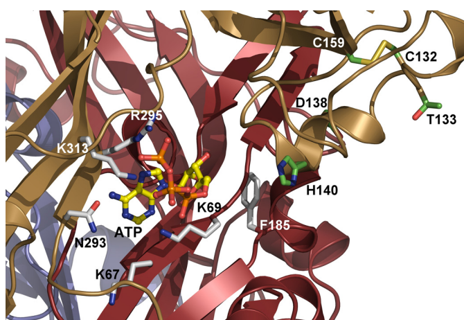
FIG. 7. Residues of the rat P2X4R potentially involved in the modulatory effects of copper and zinc cations (Wildman et al., 1999; Acuña-Castillo et al., 2000; Coddou et al., 2003, 2007). Structural model of rat P2X4R shows the location of residues Asp 138 , His 140 , Thr 133 , Cys 132 , and Cys 159 (shown as sticks) with respect to the predicted ATP-binding site. All these residues are present within the head domain of one subunit, which creates one wall of the predicted ATP-binding pocket and is probably involved in the ATP-induced conformational change. The figure was generated using PyMol v0.99 ( http://www.pymol.org ).
